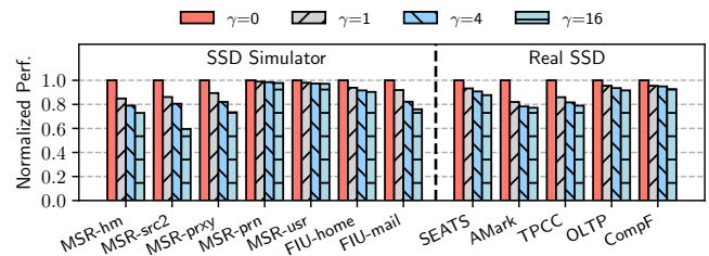
Figure 21: Performance with various \gamma (lower is better).
